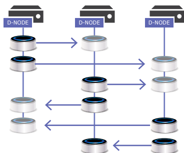
Local Disk Failover Synchronous replication of forests across local hosts using journal frames
